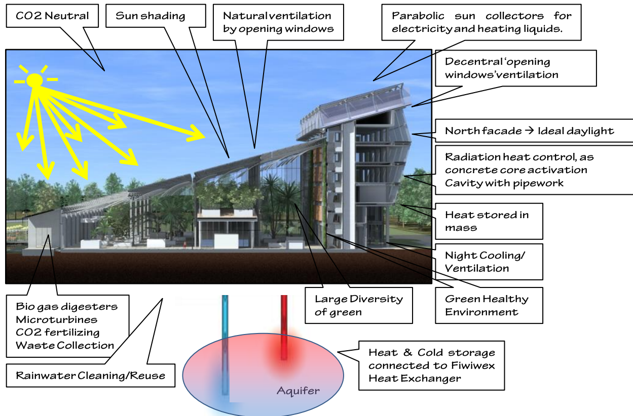
Fiwiwex Heat-exchanger
